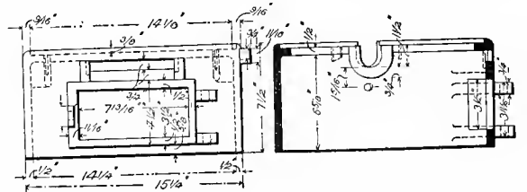
Fig. 3070a. Section of Ash-pit.
